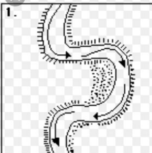
Diagram 2.6h The formation of an Ox - bow Lake.
