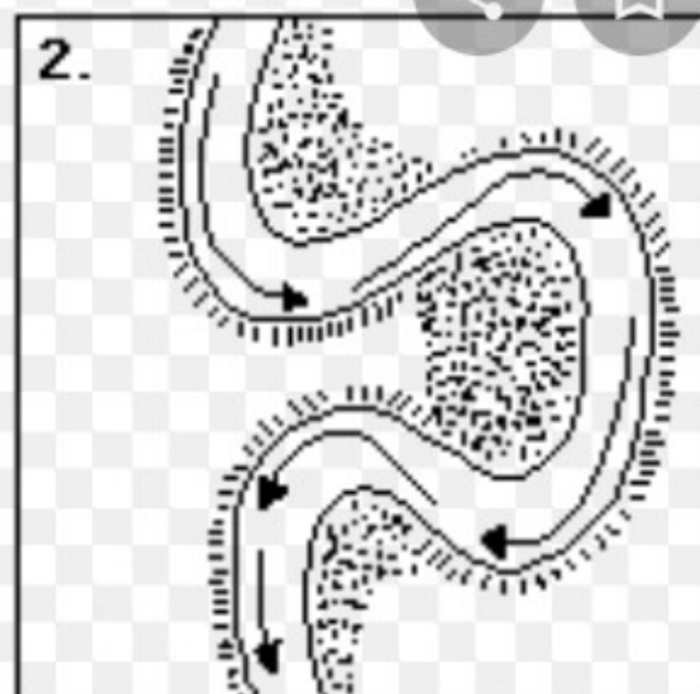
Diagram 2.6h The formation of an Ox - bow Lake.
